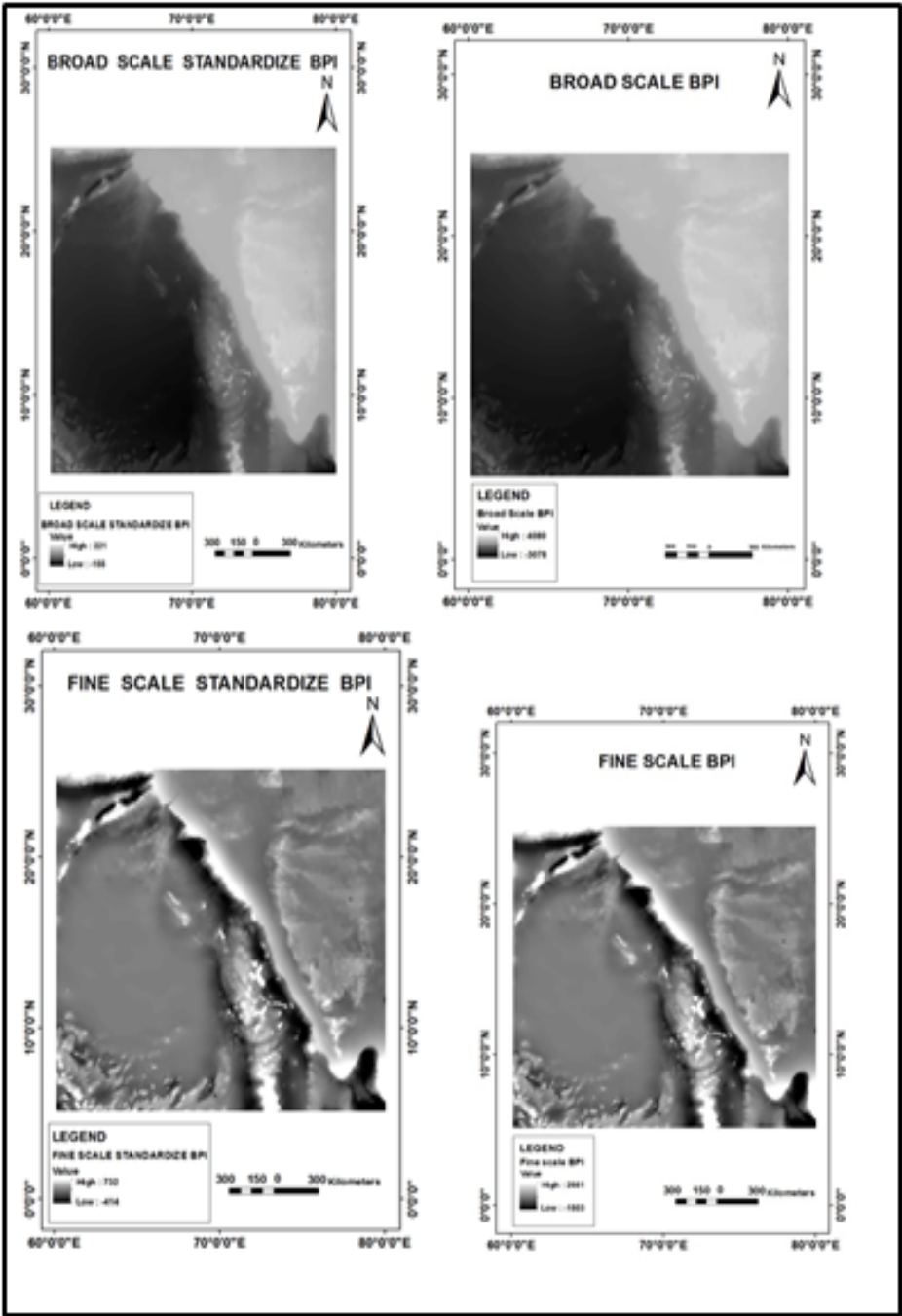
Figure 8. Maps showing the benthic terrain classification using Bathymetric Position Index (BPI) data sets at fine, broad and standardized scale
