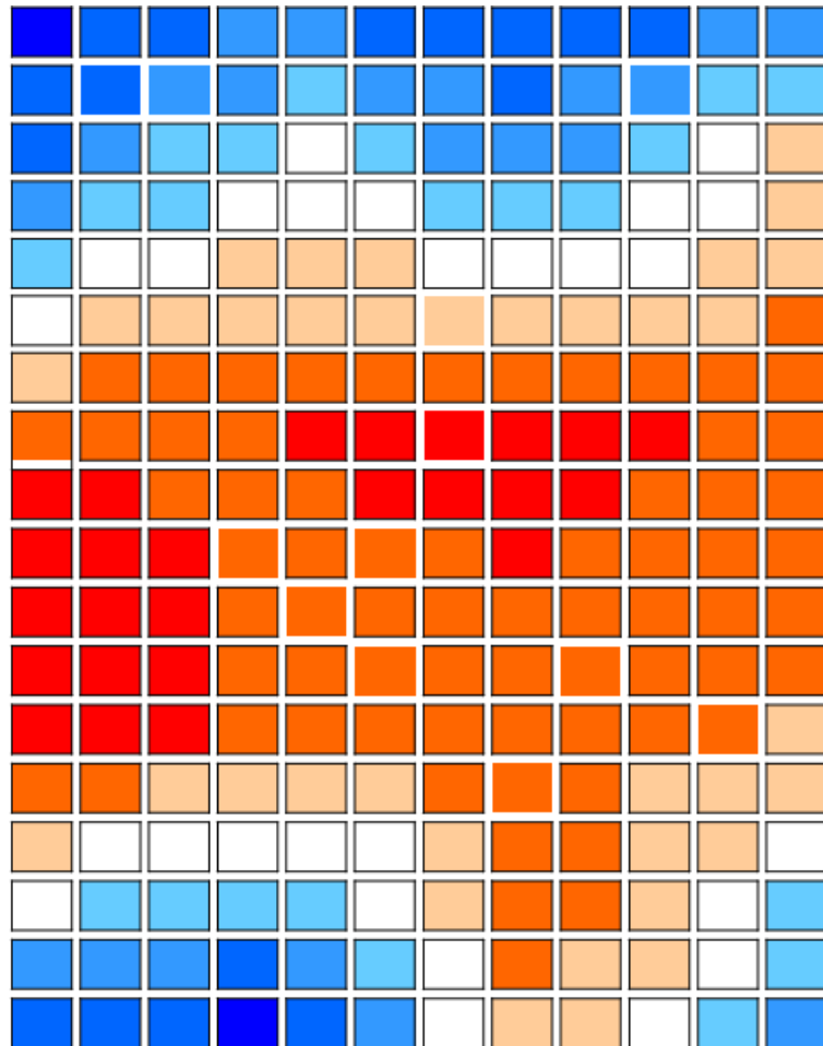
Readily available water (RAW) per experimental plot
